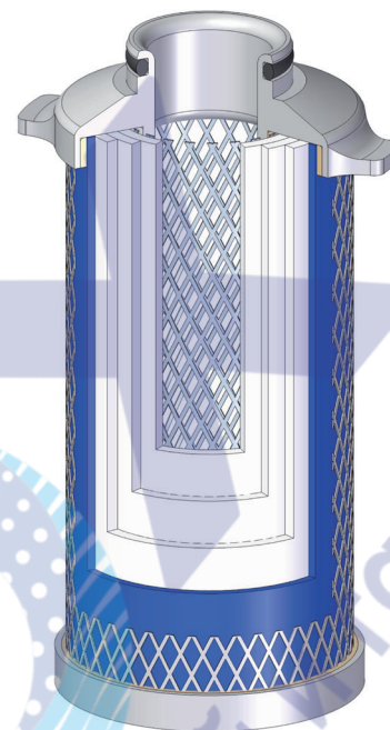
Cross section of the depth filter
